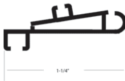
RETAINER PROFILE 2310 Part# B1.0029 Use with gasket 2261. For Anthony Model 1000 doors.
