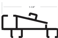
RETAINER PROFILE 2286 Part# B1.0030 Use with gasket 9536. For Anthony Model 1001 doors.
